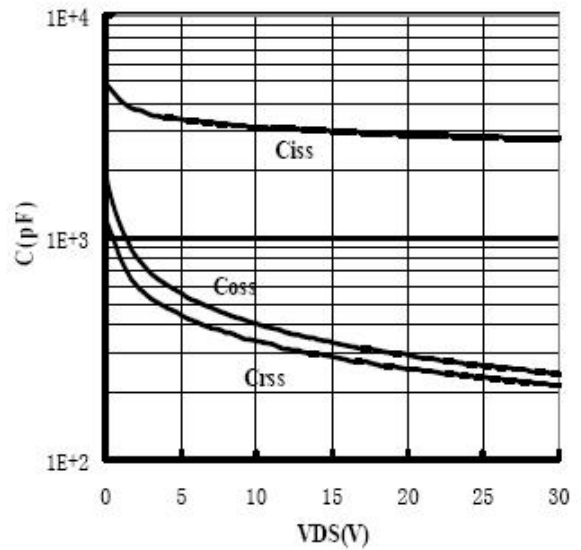
Figure 10. Capacitance Characteristics
