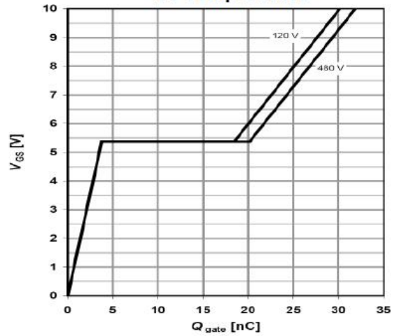
Figure 10. Gate charge
