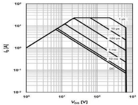
Figure 4. Maximum Safe Operating Area for TO-251, TO-252 @ 80°C
